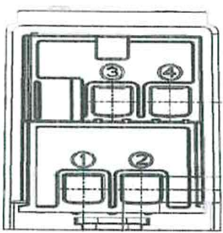
Figure 1. Terminals Configuration
